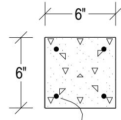
#3 REBAR (TYP.) 6" x 6" POST SECTION VIEW
