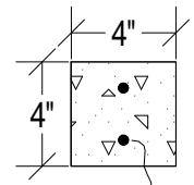
#3 REBAR (TYP.) 4" x 4" POST SECTION VIEW
